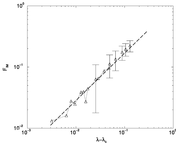
Fig. 4. Log–log plot of the fraction of infected nodes F_{IM} as function of \lambda - \lambda_c for (\rho = 0.2, T = 1) , with \lambda_c = 0.935 . The dashed line is a fit to the form F_{IM} \sim (\lambda - \lambda_c)^\beta , with exponent \beta = 0.773 .
